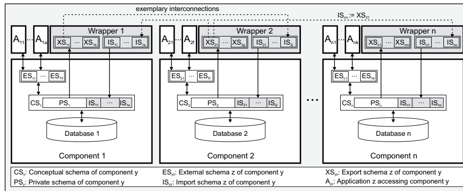
Fig. 1. DÍGAME Architecture
